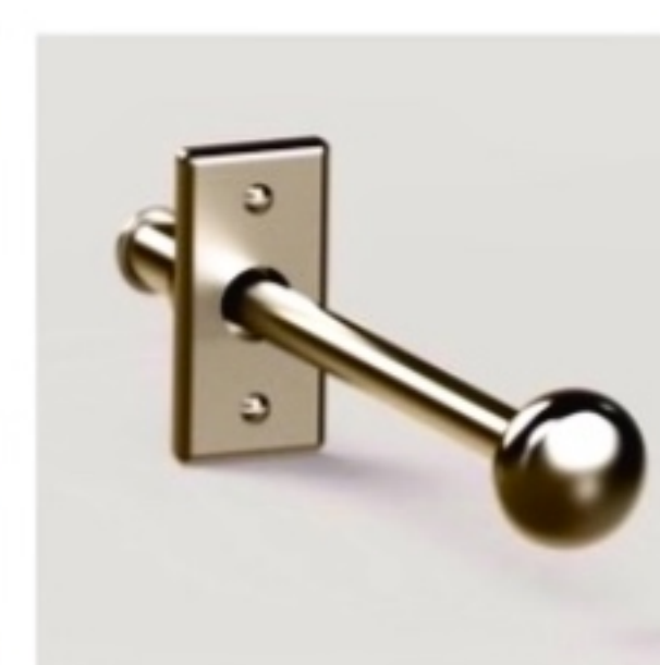
8668GR Garment Rod Rectangular Plate - Face Fixed
